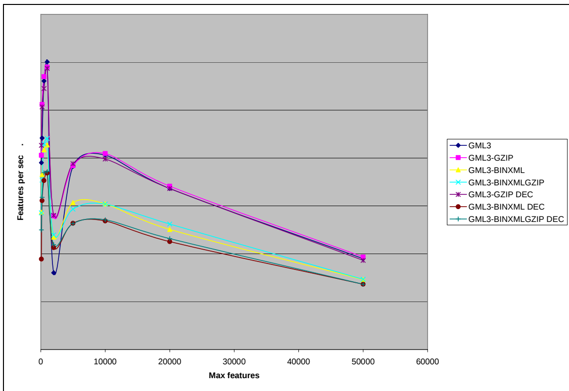
Figure 8.2.3-1 — 100 MBPS LAN elevp_elev_1m Feature Count Vs. Rate
