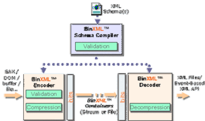
Figure 6.1.2-1 — BinXML Code/Encoder Workflow.
