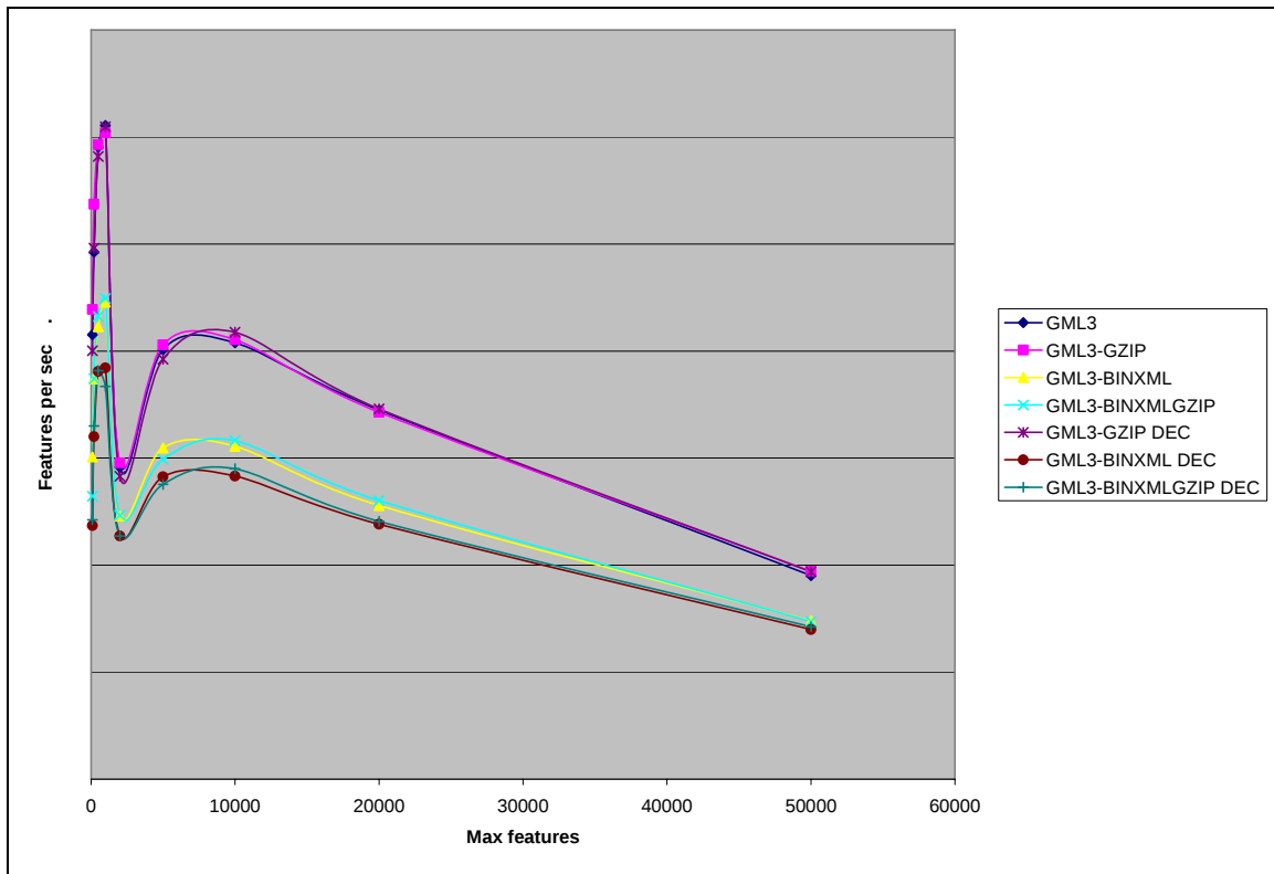
Figure 8.1.3-1 — Local Server elevp_elev_1m Feature Count Vs. Rate.
