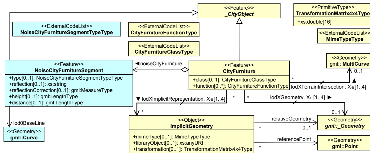
Fig. 66: CityGML noise application schema – city furniture model (light yellow=CityGML standard, light blue=CityGML Noise ADE) (source: Institute of Geodesy and Geoinformation Uni Bonn).
