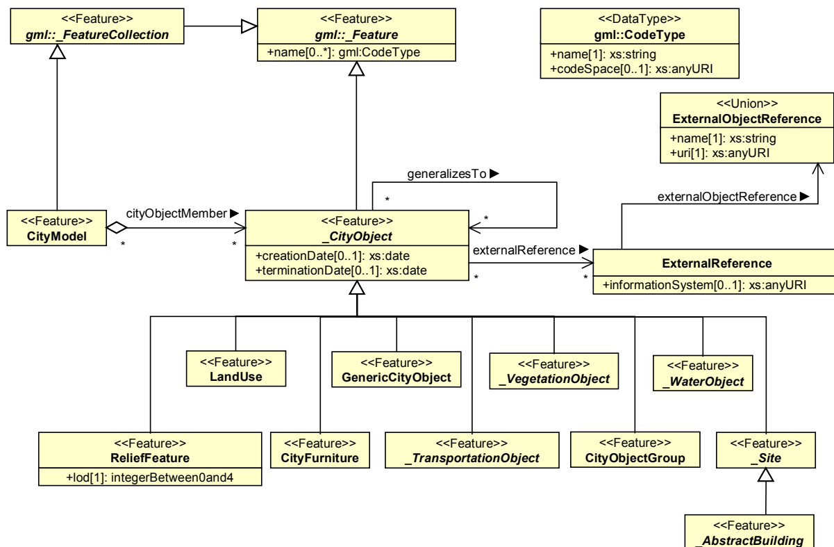
Fig. 20: UML diagram of the top level class hierarchy of CityGML. The bracketed numbers following the attribute names denote its multiplicity: the minimal and maximal number of occurrences of the attribute per object. For example, a name is optional (0) in the class Feature or may occur multiple times (star symbol), while a _CityObject has none or at most one creationDate . A ReliefFeature has exactly one occurrence of the attribute LOD .
